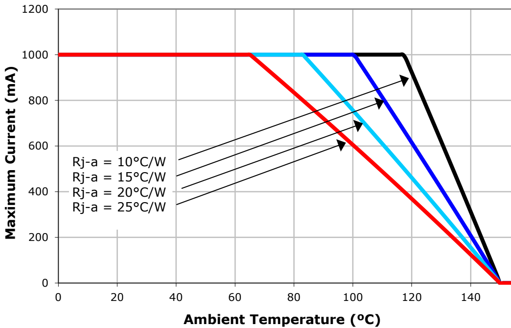
Figure 7: XB-D current de-rating curve
