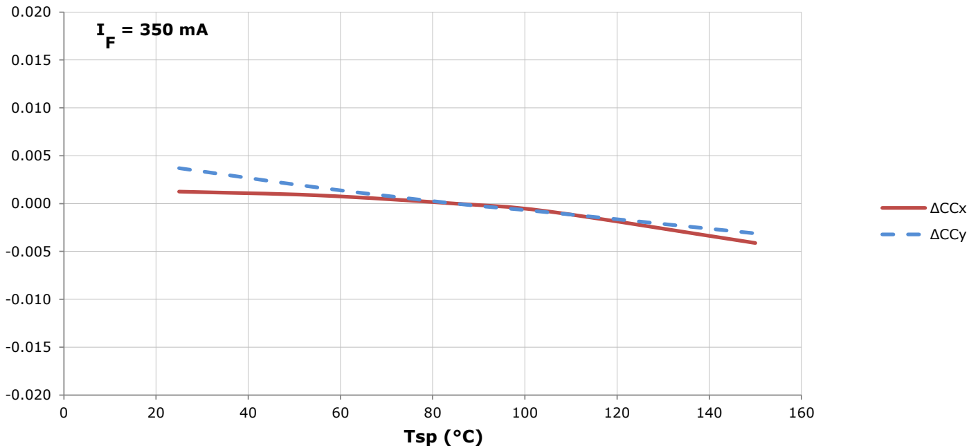
Figure 3: XLamp XB-D LED color shift vs. solder point temperature
